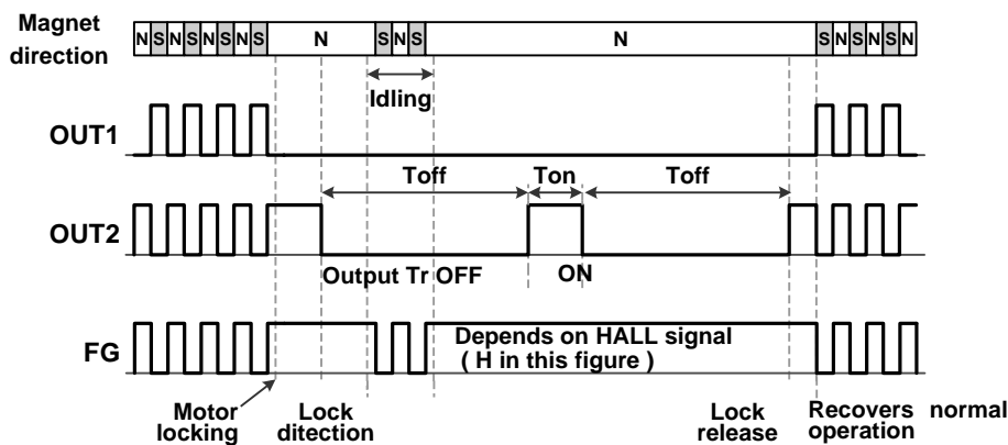
Figure 25. Lock protection timing chart
