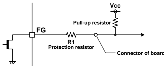
Figure 30. Protection of FG terminal
